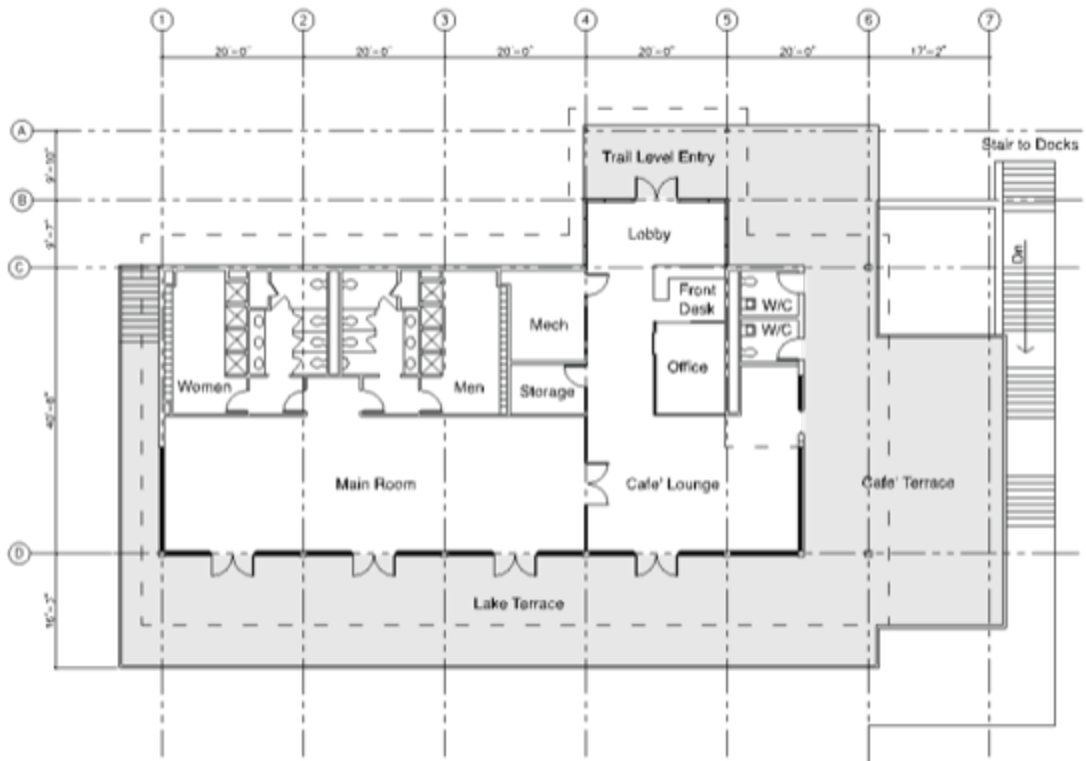
Waller Creek Boathouse Floor Plan scale: 1/8" = 1'-0"
